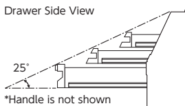
Drawer Side View
